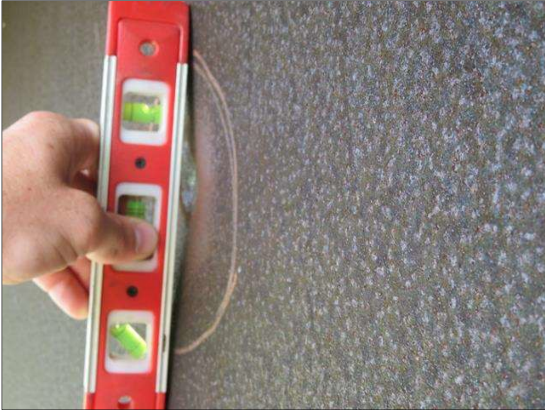
Span 2 Beam 1: 4" DIAMETER X 3/4" DEEP INDENTATION IN BEAM 1 IN SPAN 2 WEB LOCATED 17" FROM TOP FLANGE AND OVER RIGHT WEST BOUND THRU LANE.
